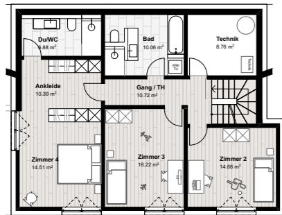
Erdgeschoss 1/00
