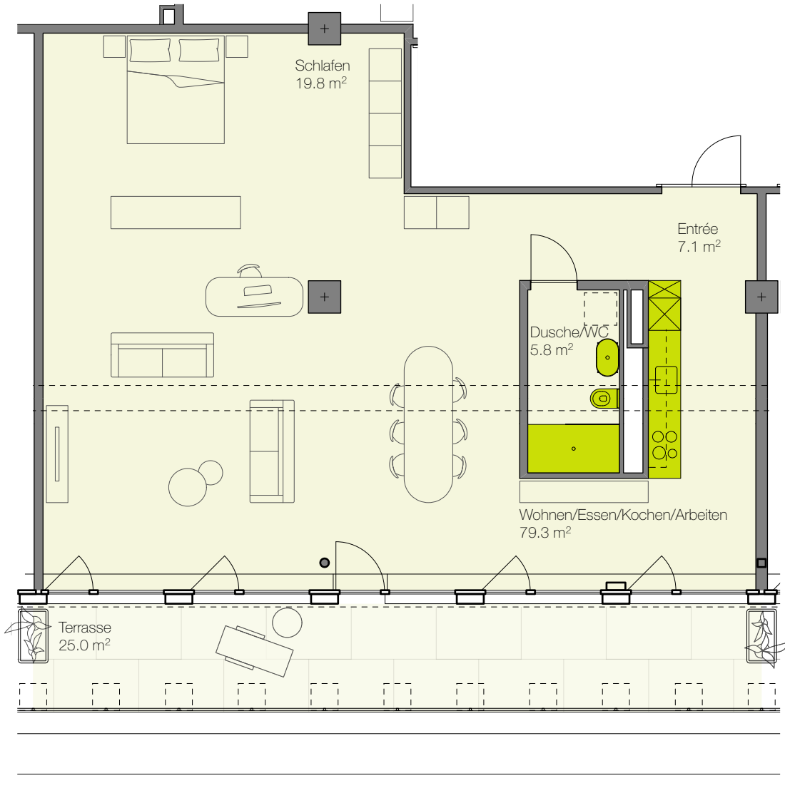
Grundriss Attikageschoss Mst. 1:100
