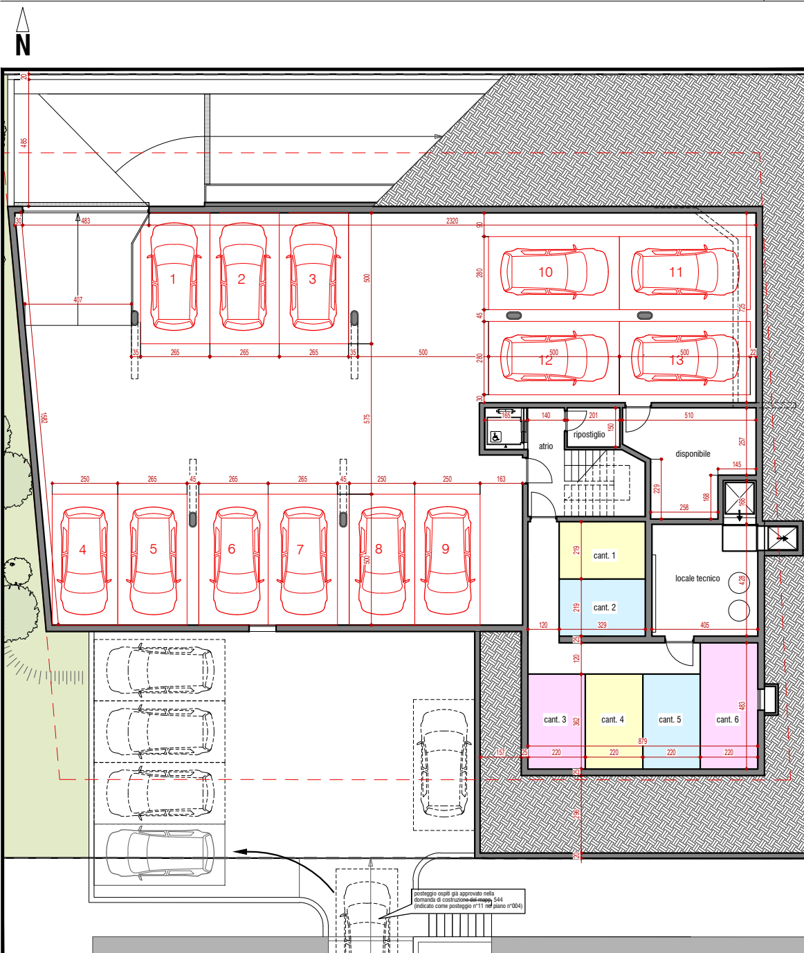
Piano Interrato 1:200
