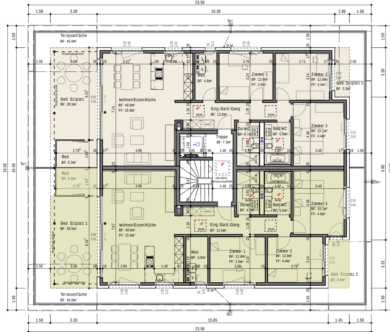
Attikageschoss links A 4.5-Zi-Whg. NF 106m²/BGF 130m²
