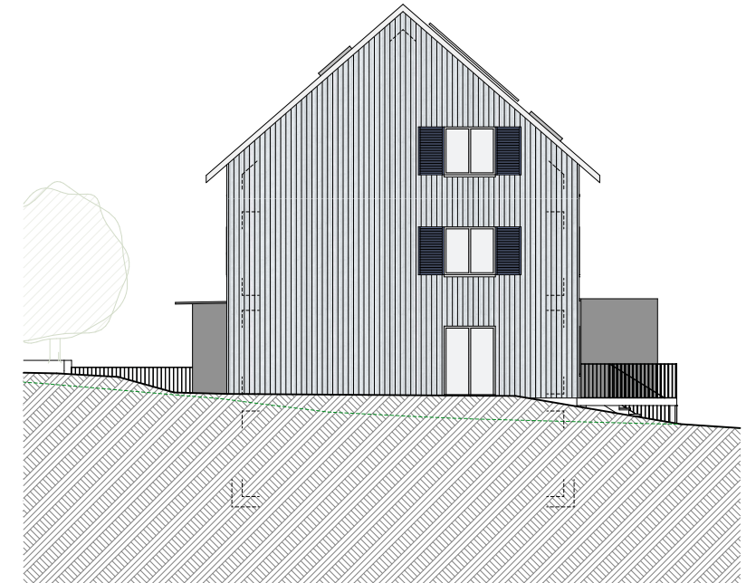
Fassade West
