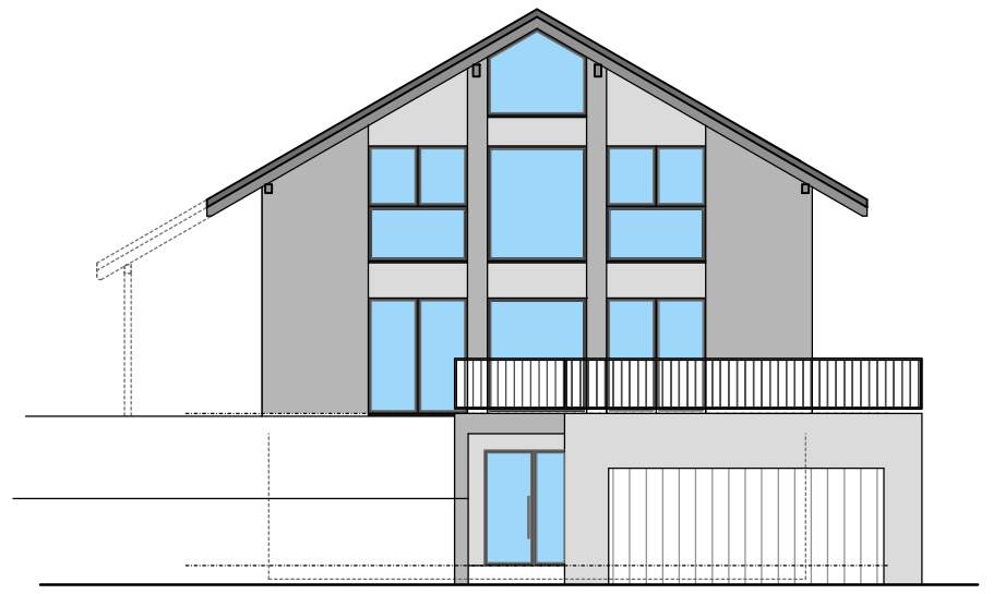
Fassade SUED
