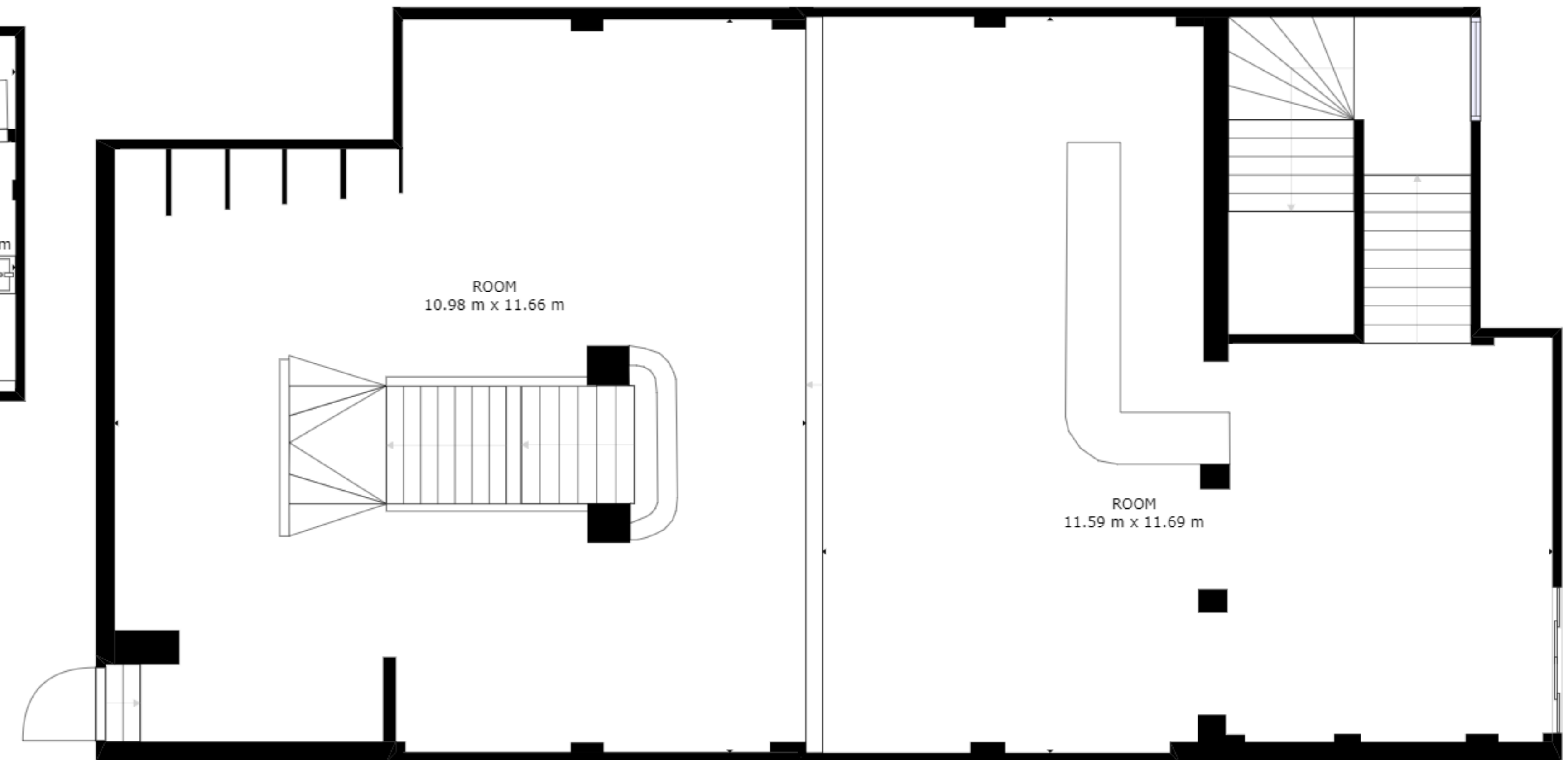
FLOOR 2
