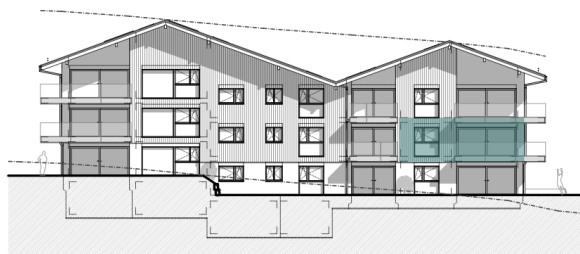
SITUATION - FACADES
