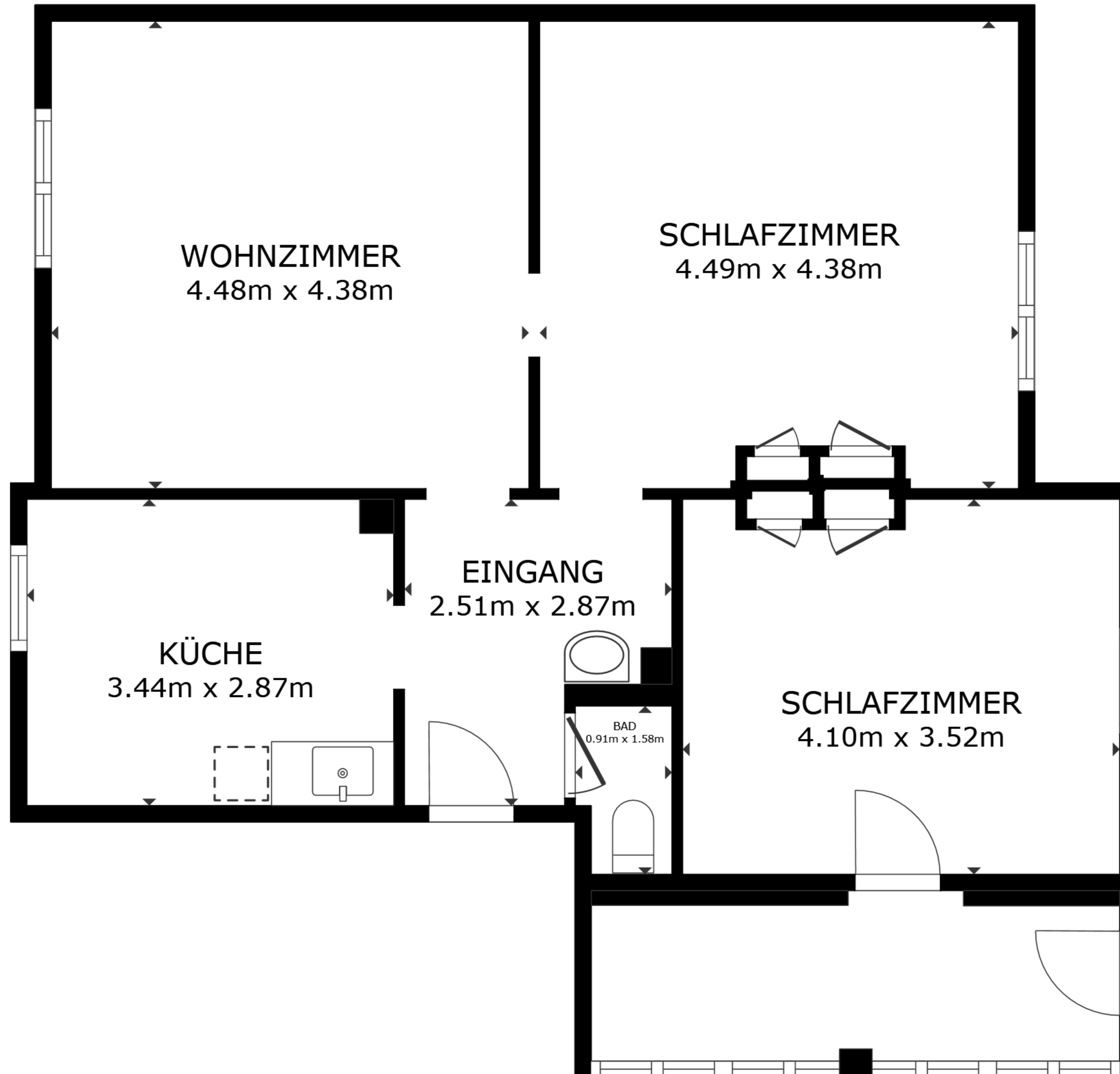
FLOOR PLAN
