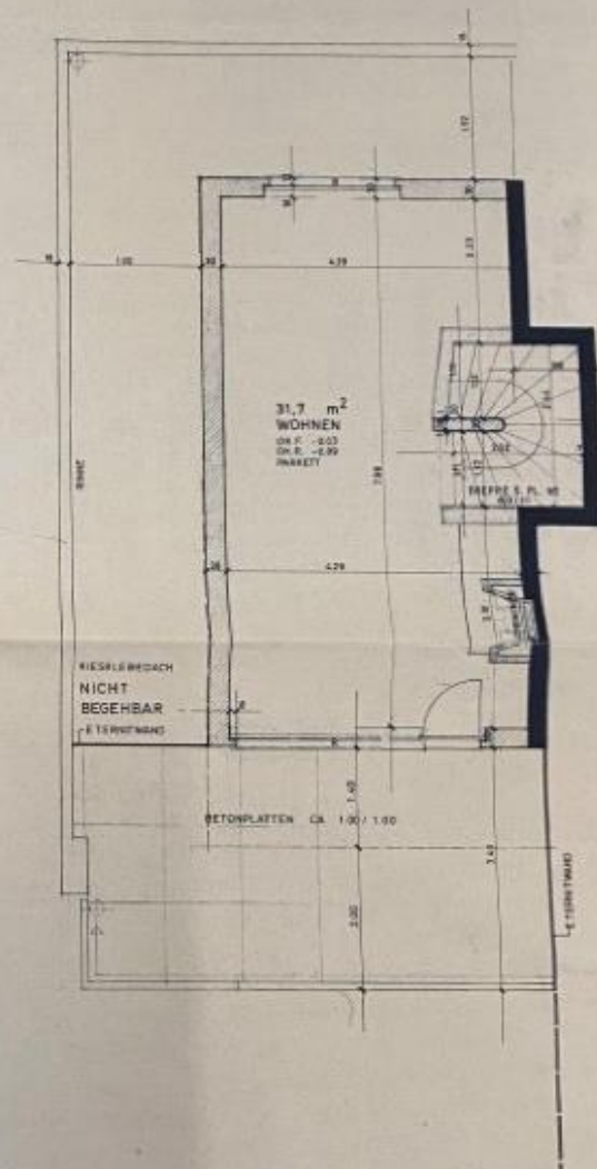
ATTIKA
