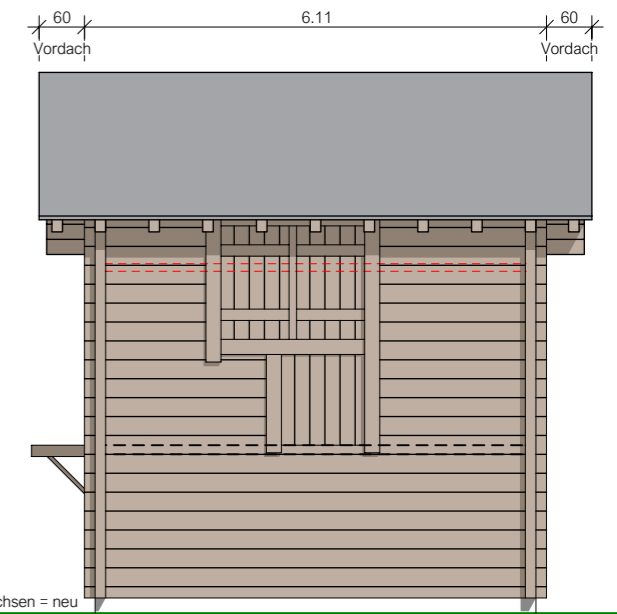
Fassade Nord-West
