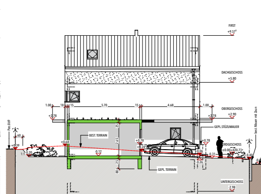
B/2 NORDEN 1:100
