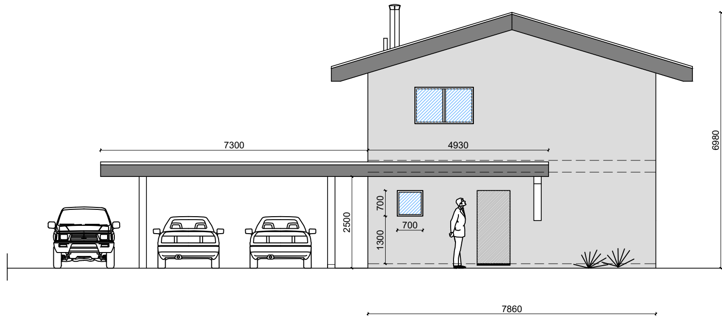
LOT A COUPE C-C
