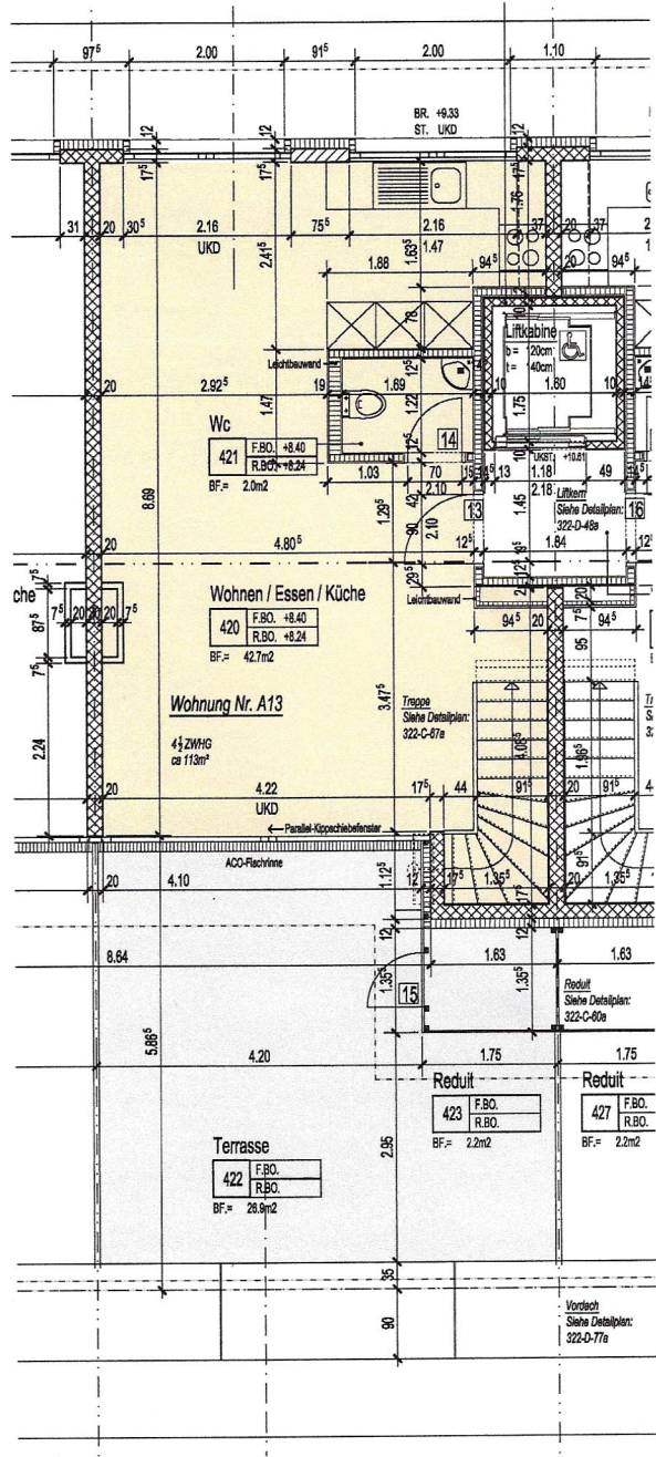
Attikageschoss
