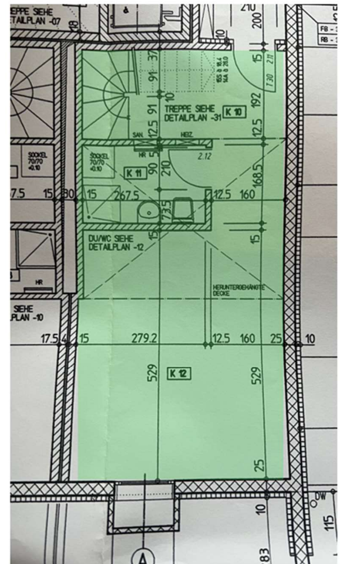
Plan UG
