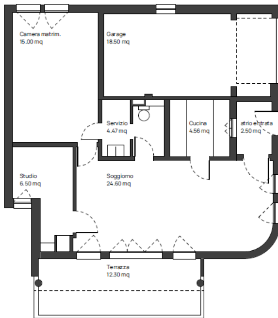
Piano superiore / Obergeschoss
