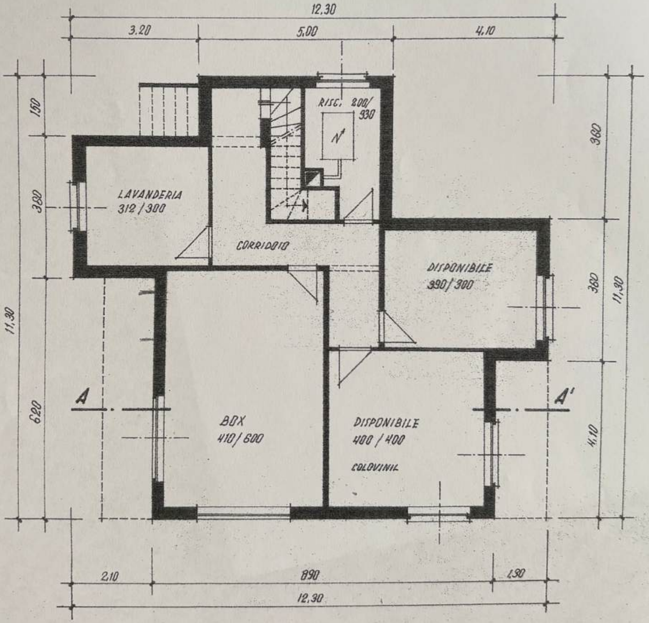
PIANO CANTINATO
