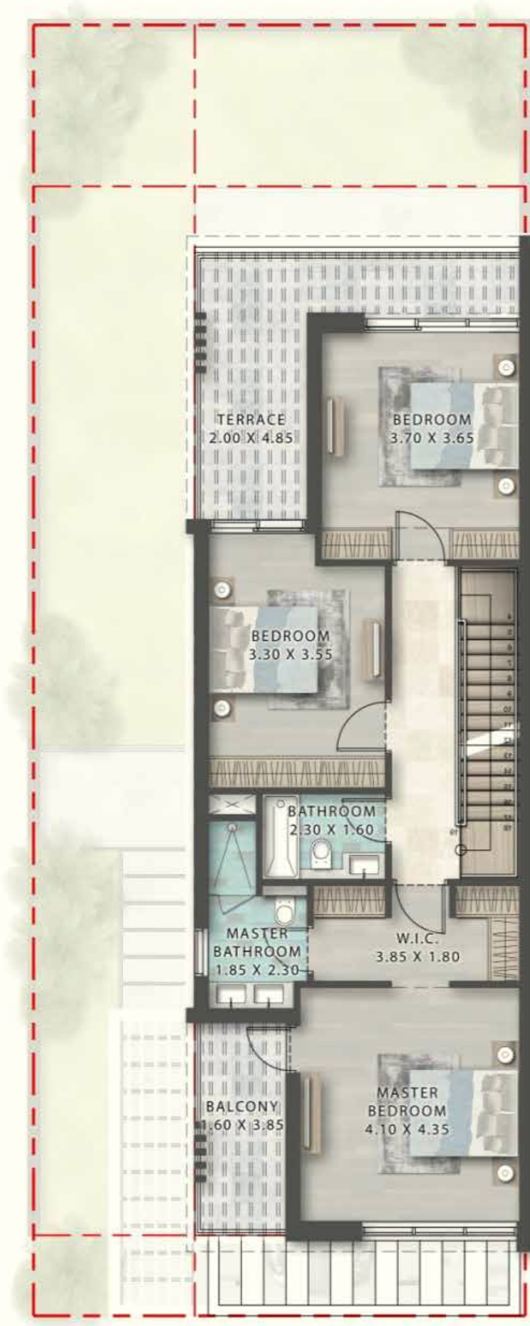
FIRST FLOOR
