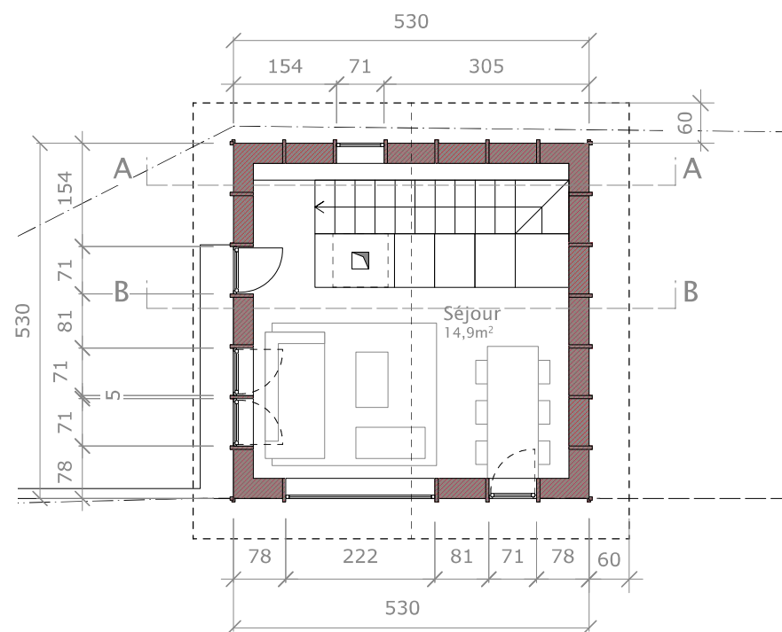
PLAN REZ
