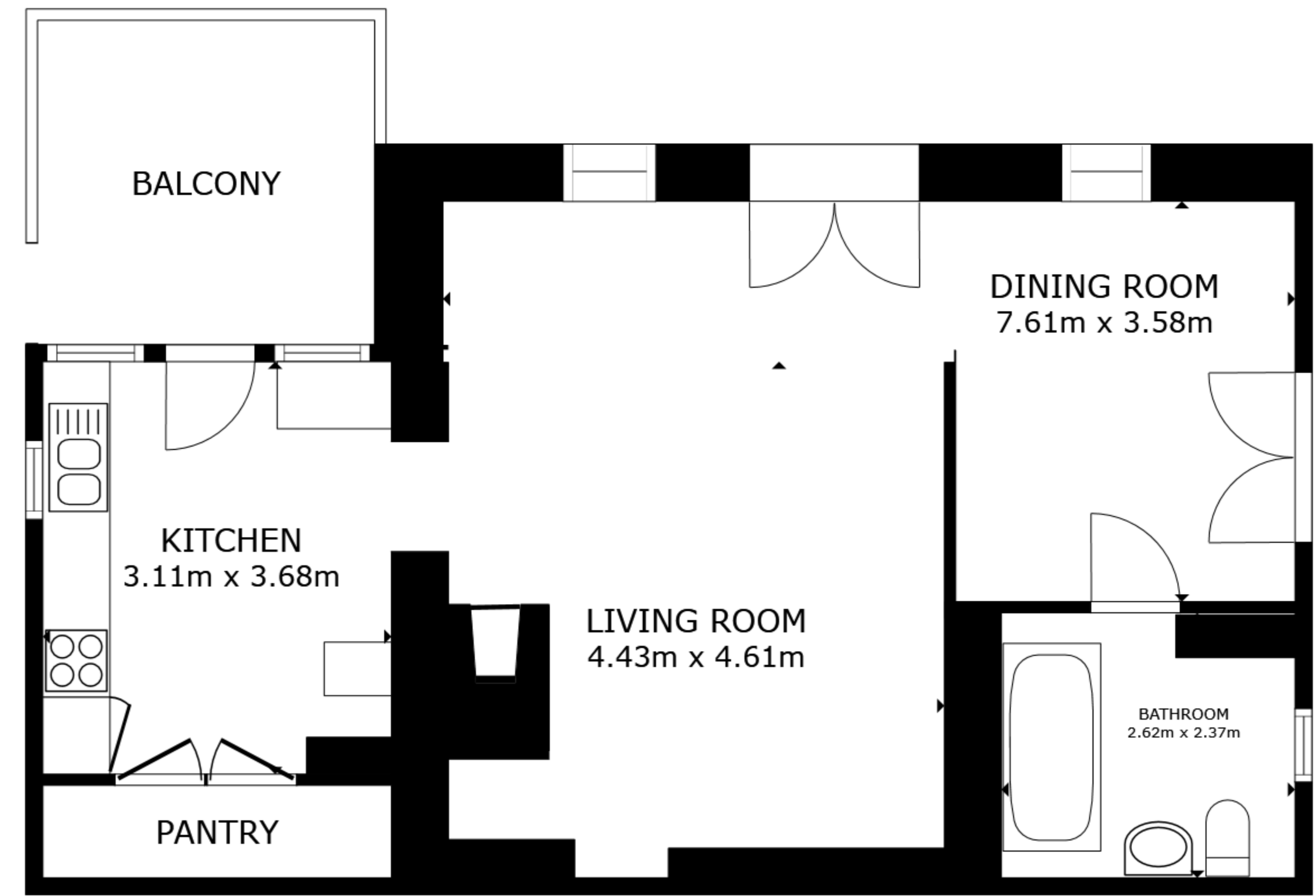
FLOOR 2
