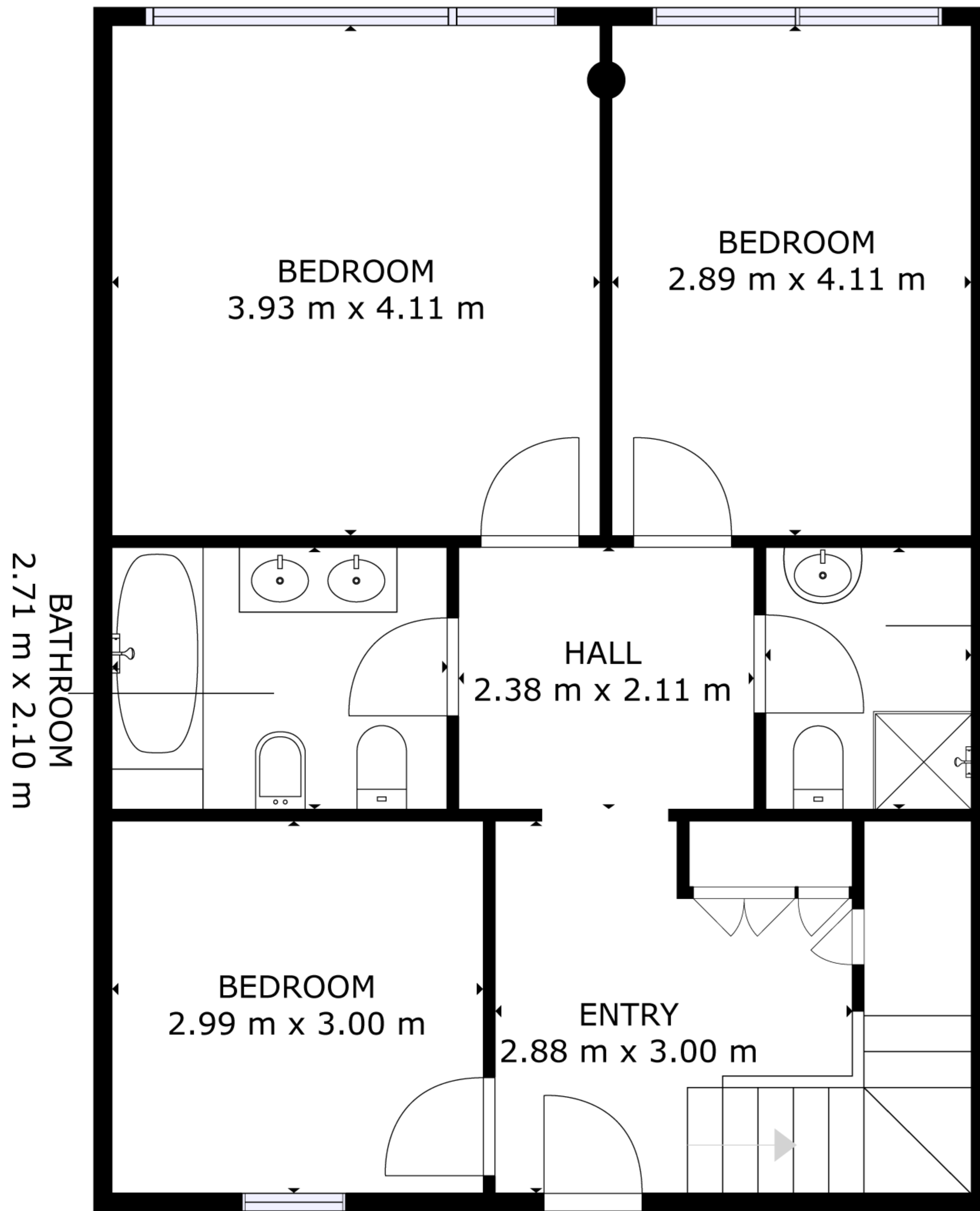
FLOOR 1
