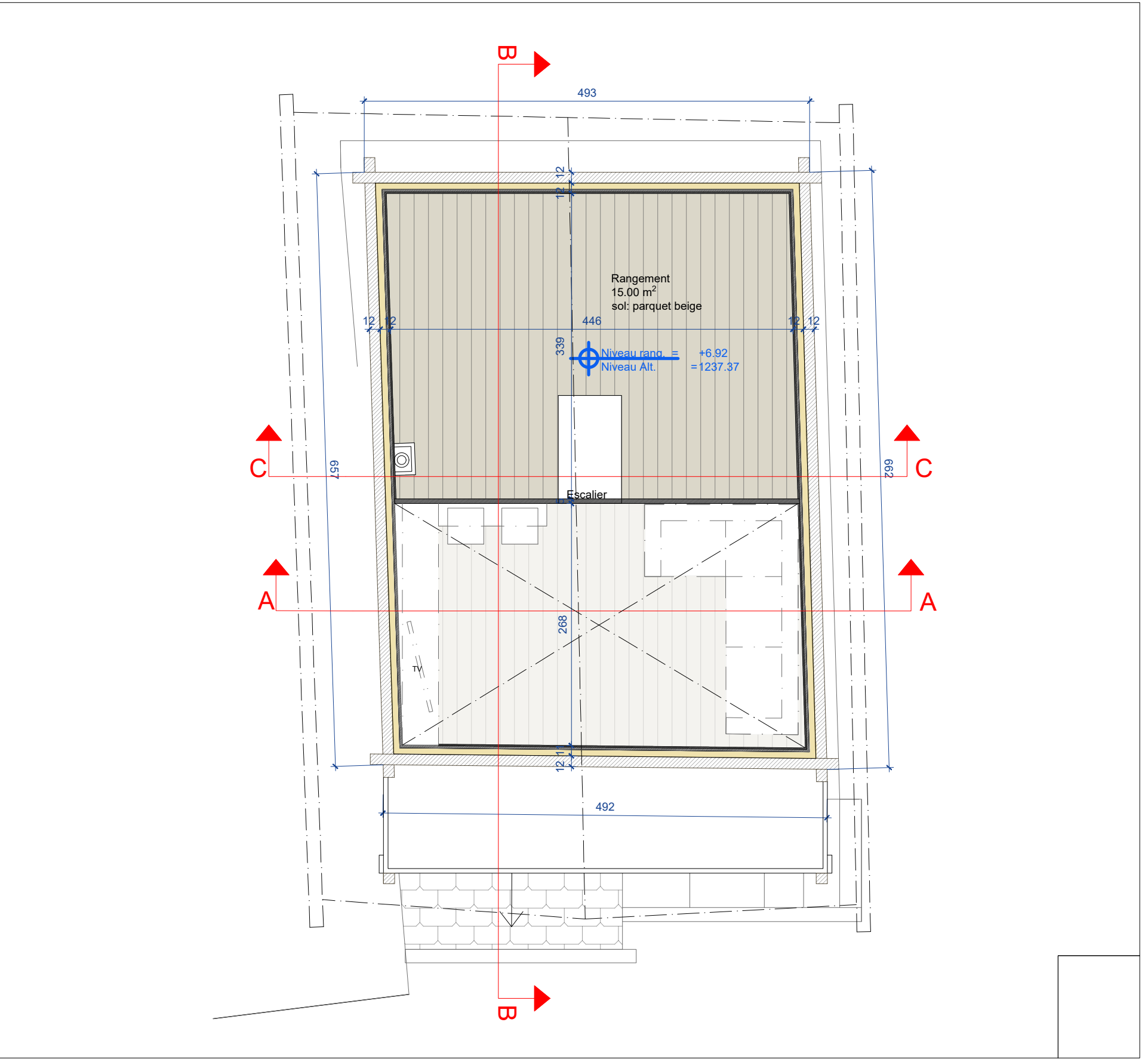
Plan Combles
