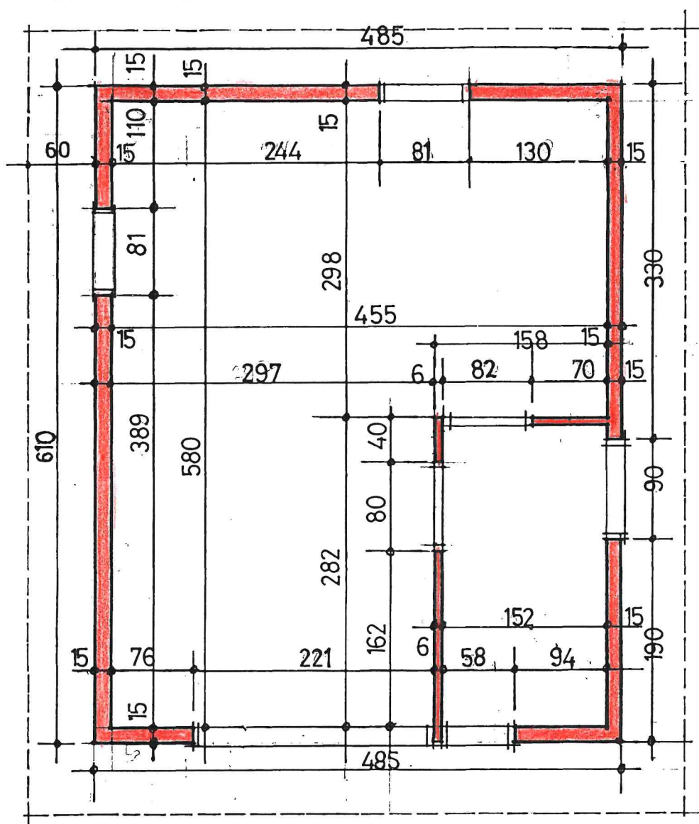
PLAN PAVILLON
